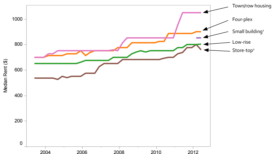
Median Rent by Building Type, Jun '03 to Jun '12
